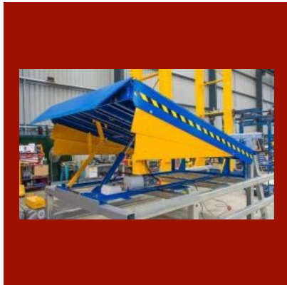
Mechanical Dock Leveler
